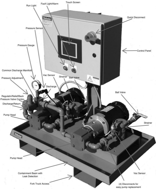
The above SPM pump set is sitting on a 36" x 24" containment basin. Dimensions may vary depending on model.
