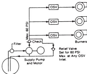
Figure 3. Supply Pump Systems — Multi Level
