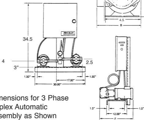
SPMV DUPLEX AUTOMATIC SUPPLY UNIT
