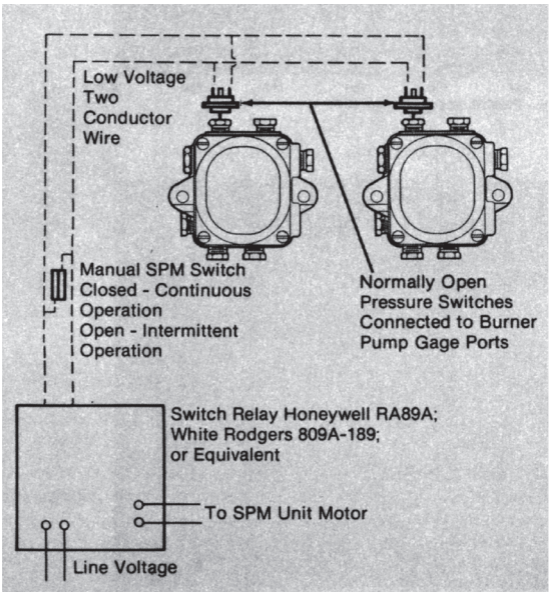
Wiring for intermittent operation
