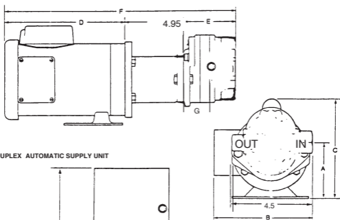
SPMV SINGLE SUPPLY UNIT
