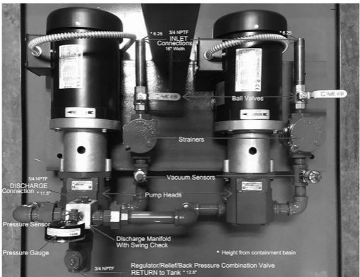
The above SPM pump set is sitting on a 36" x 24" containment basin. Dimensions may vary depending on model.
